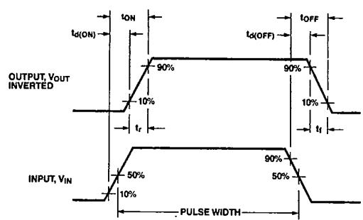
Figure 2 Switching Waveforms
