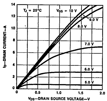
Figure 3 Output Characteristics
